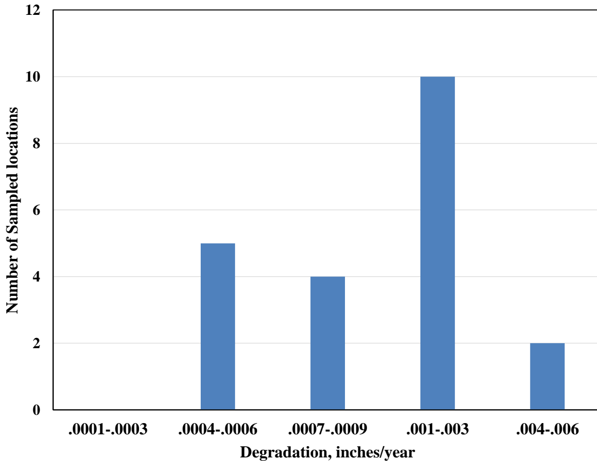
Figure 7-1. Degradation rate, inches/year for samples from BVVPOA
