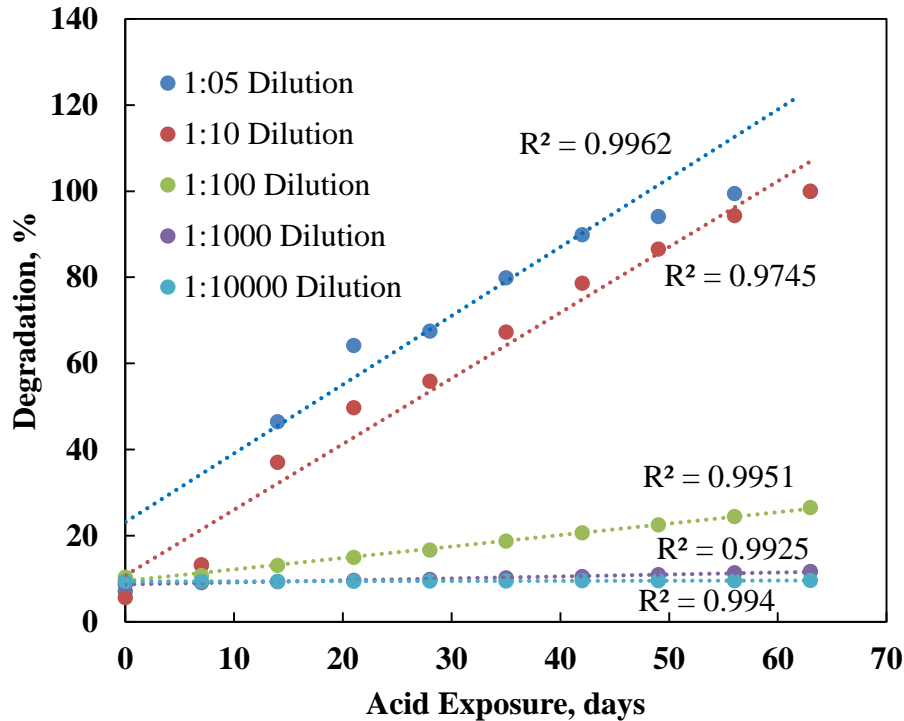
Figure 6-5. Phase III acid test results showing linear rate of degradation for all dilutions
